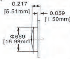
Nozzle without gasket type
