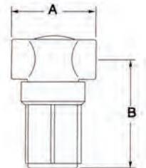
Polypropylene strainer body
