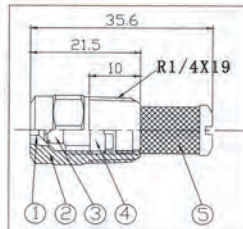
1.Orifice 2.Body 3.Cyclone Core 4.Plug 5.strainer mesh
