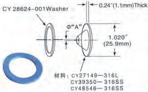
nozzle without gasket type
