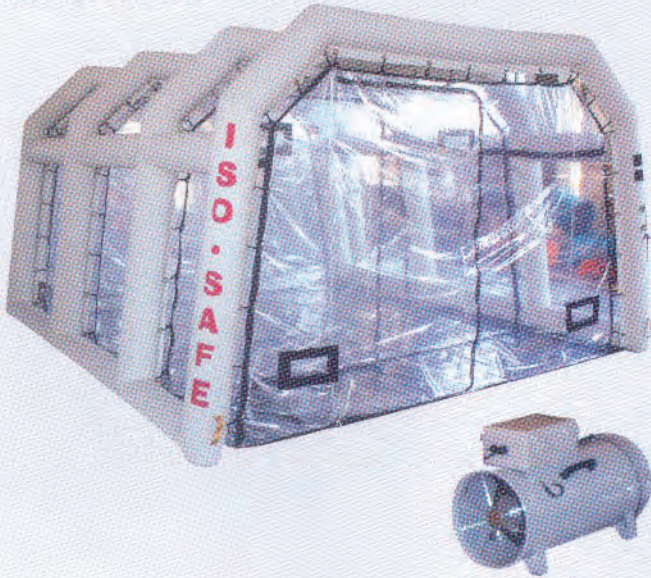
HEPA Filter
